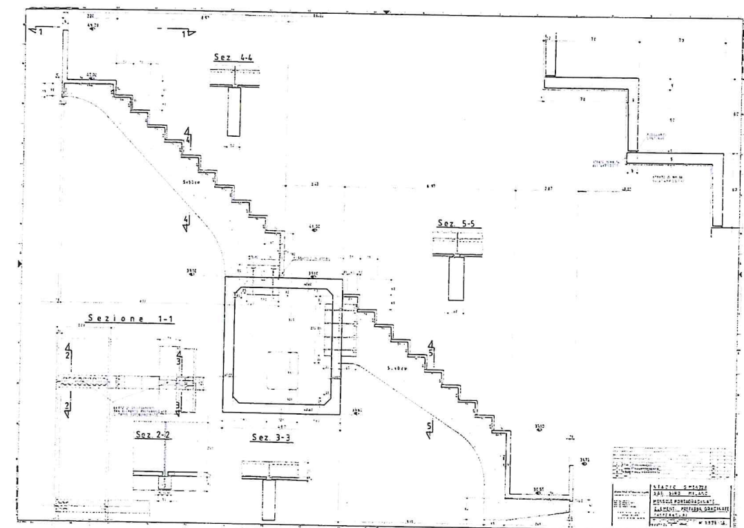
Fig. 10: Mensole portagradinate
